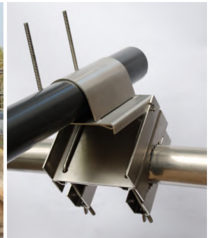
200506 Rail mounted hinged pipe bracket for 50 mm PVC pipe on Universal Bracket 200505.
