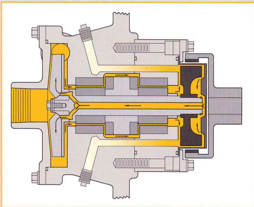
Our unique forced product circulation system lubricates our bearings and provides cooling to alleviate heat rise induced by magnetic eddy-current in the containment can.
