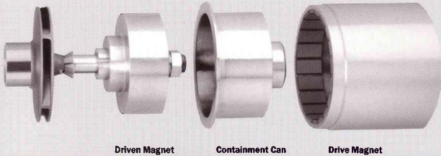
Driven Magnet
